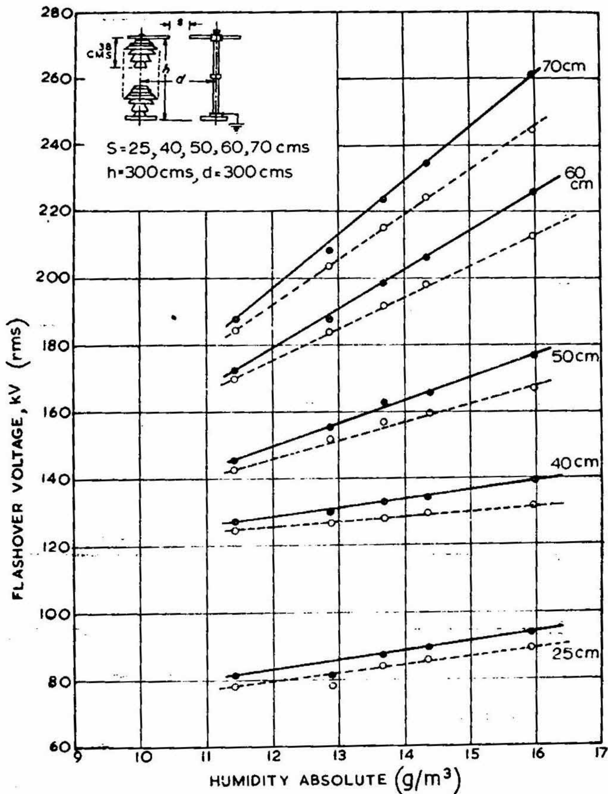
FIG. 3. Effect of humidity on breakdown voltage of rod gaps at 20^\circ \text{C} . —●— experimentally obtained data; ...○... data corrected by applying standard humidity correction.
