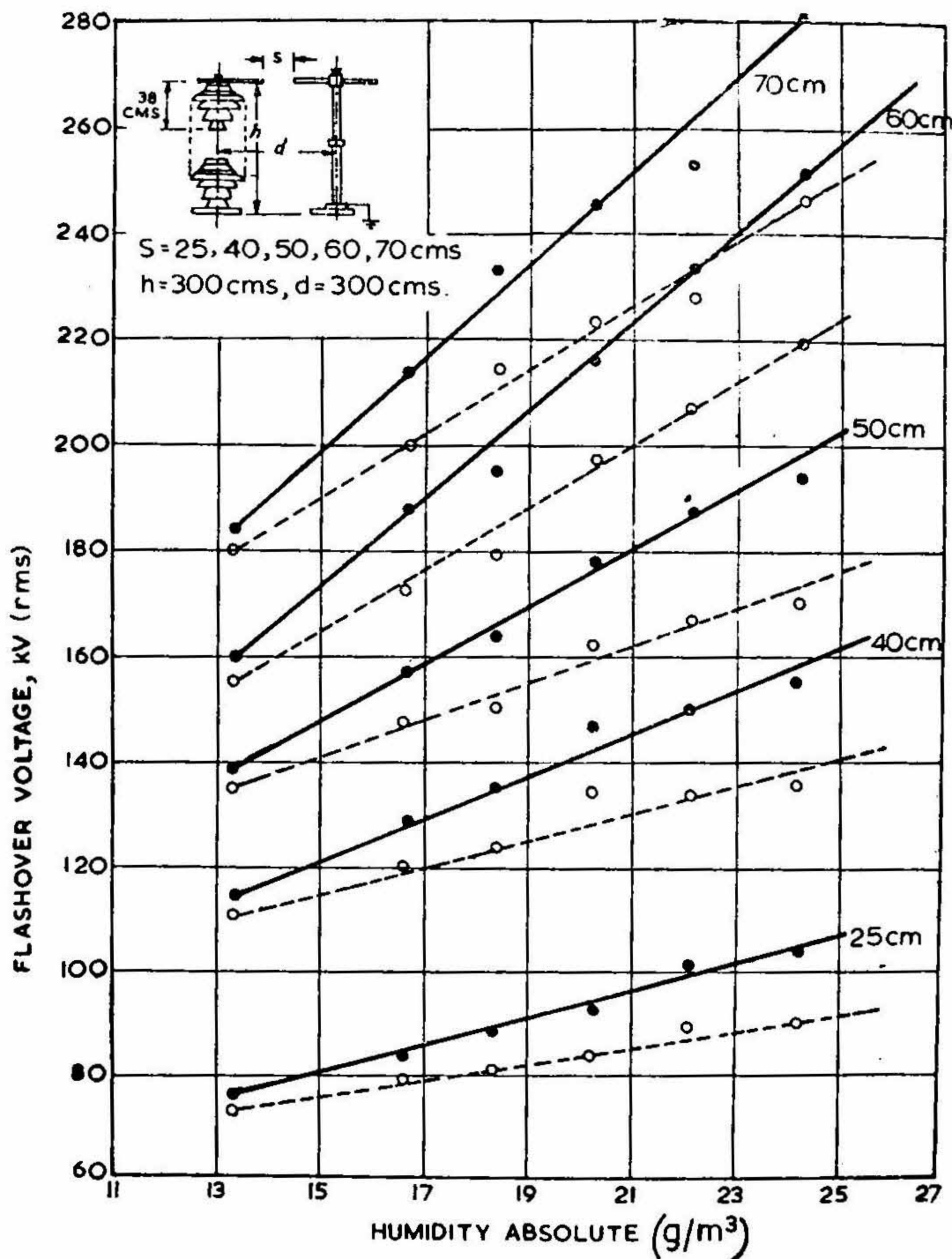
FIG. 4. Effect of humidity on breakdown voltage of rod gaps at 27° C.
