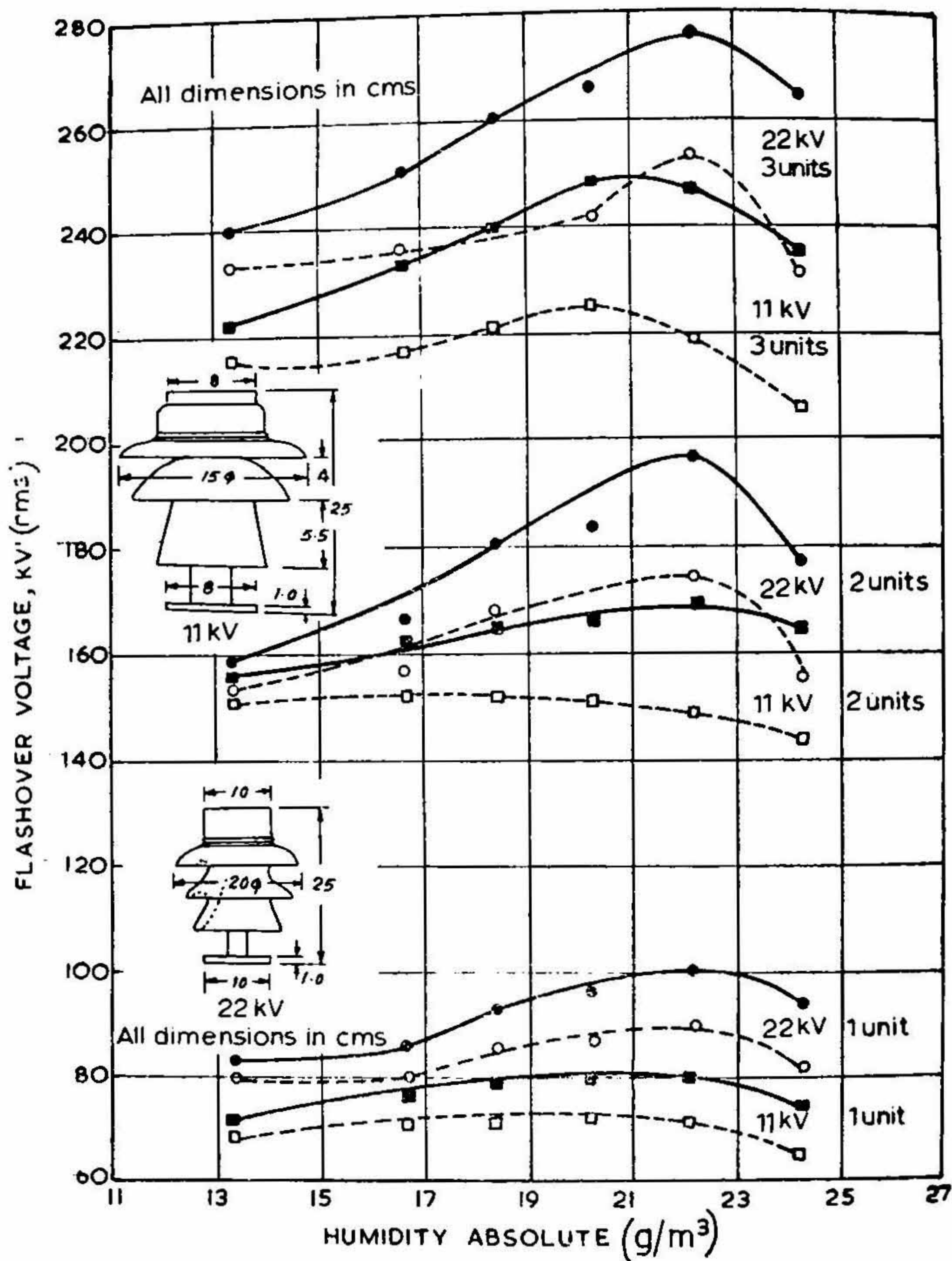
FIG. 8. Flashover voltage of variation with humidity for post insulators at 27° C. —●— experimental curve; ...○... corrected curve.
