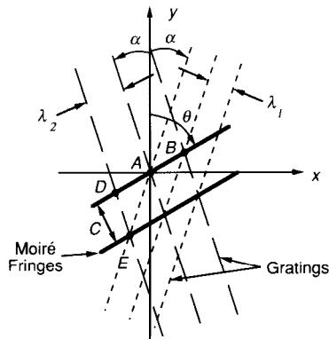
Figure 16.3. Geometry used to determine spacing and angle of moiré fringes between two gratings of different frequencies tilted with respect to one another.
